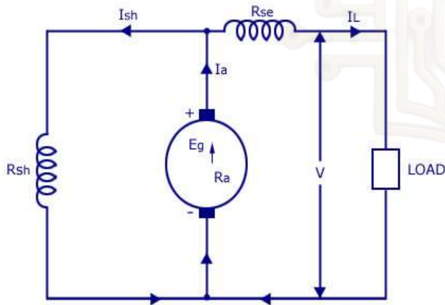
Short Shunt Compound (a)
