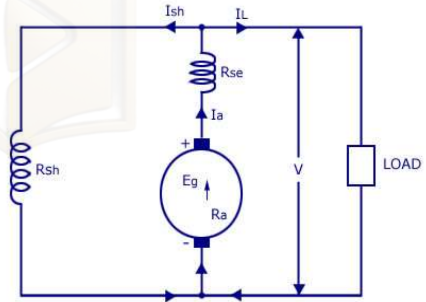
Long Shunt Compound (b)
